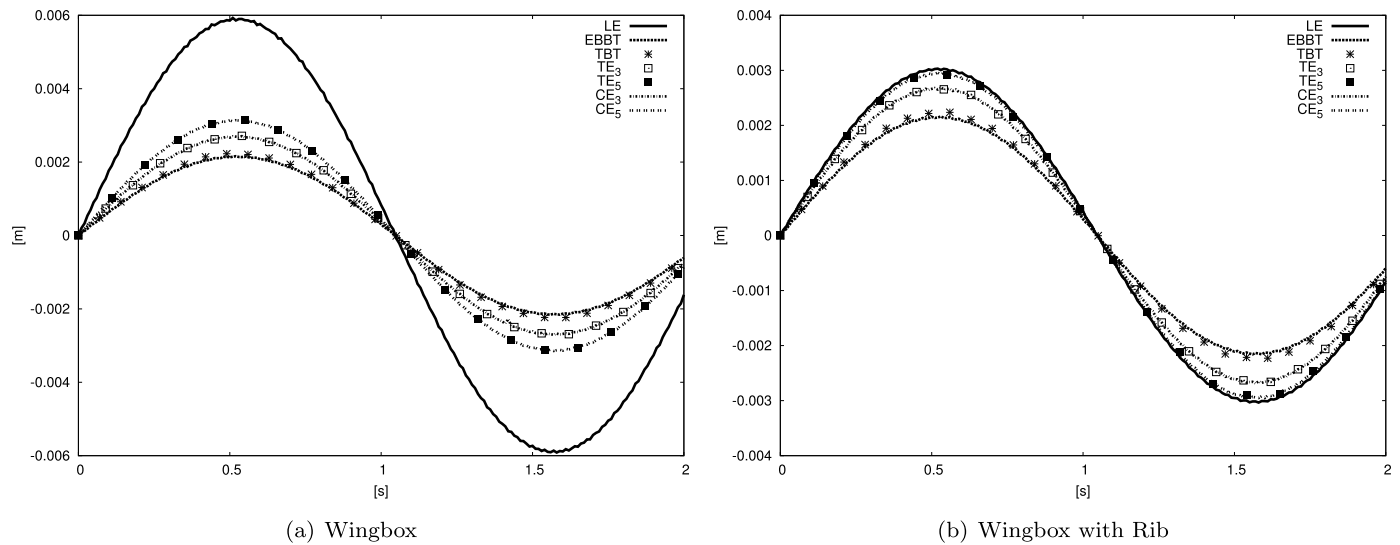
Fig. 5. Time dependent transverse displacement for various theories, wing-box model, sinusoidal loading case.
