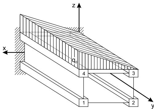
Fig. 7. Load distribution on the cross-section.
