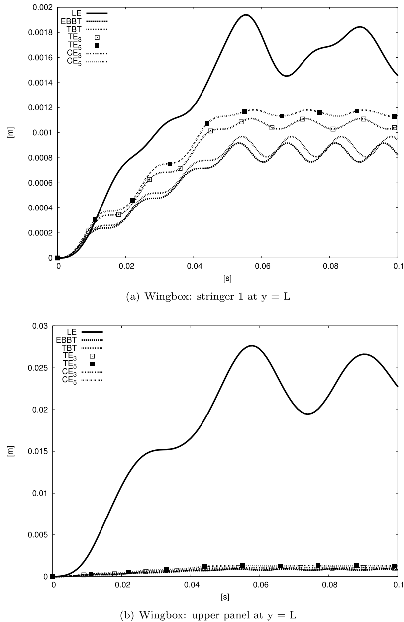
Fig. 8. Time dependent transverse displacement for various theories, wing-box model, linear loading case.
