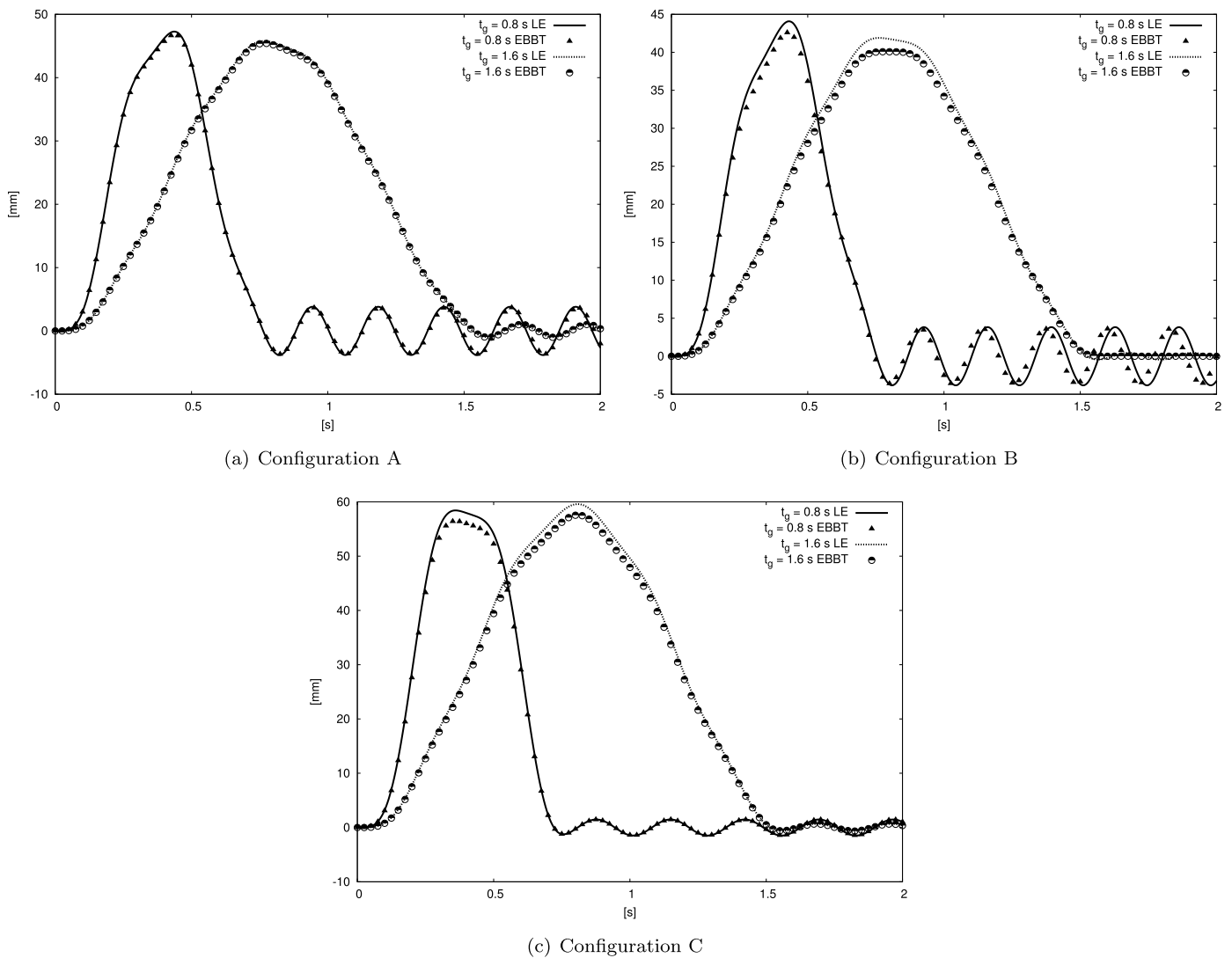
Fig. 13. Time-dependent transverse displacement at the trailing edge of the wing tip for t_g = 0.8 s and t_g = 1.6 s, various configurations of the wing subjected to gust loads.
