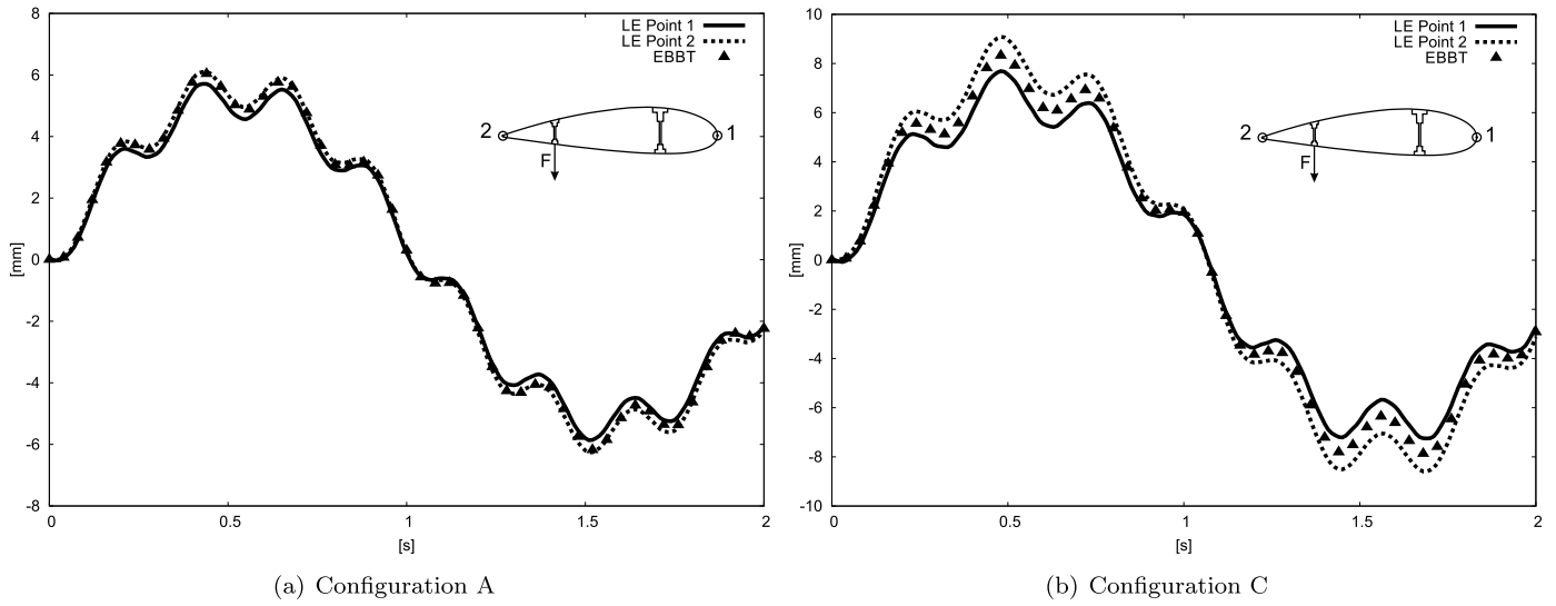
Fig. 12. Time-dependent transverse displacement at the tip for various theories. Configurations A and C of the wing subjected to sinusoidal load.
