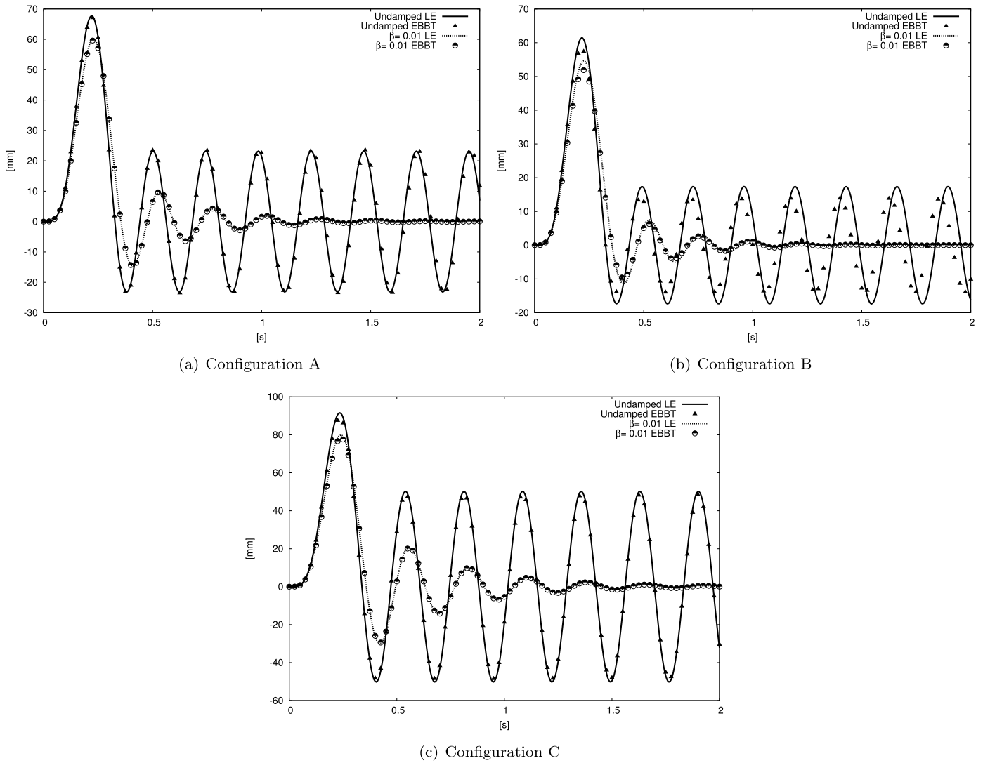
Fig. 14. Time-dependent transverse displacement at the trailing edge of the wing tip for t_g = 0.4 s in the case of the undamped and damped system, various configurations of the wing subjected to gust loads.
