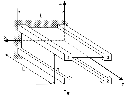
Fig. 4. Application point of the sinusoidal load, wing-box model.
