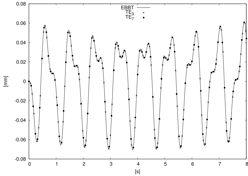
Fig. 3. Transverse displacement at the mid-span section for various theories. Square beam under sinusoidal load.
