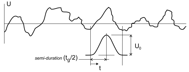
Fig. 2. One-minus-cosine discrete gust idealization.
