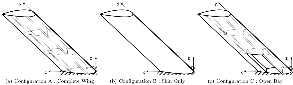
Fig. 10. Wing configurations.
