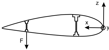
Fig. 11. Application point of the harmonic force on the cross-section.
