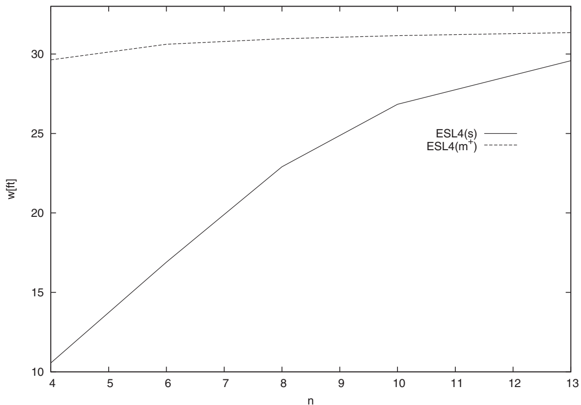
Fig. 7. Scordelis-Lo problem. Thickness ratio t/R = 0.001 . Transversal displacement w [ft] at the point B of the midsurface S by varying the mesh n \times n .
