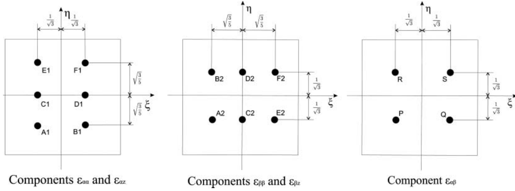
Fig. 2. Tying points for MITC9 shell finite element.
