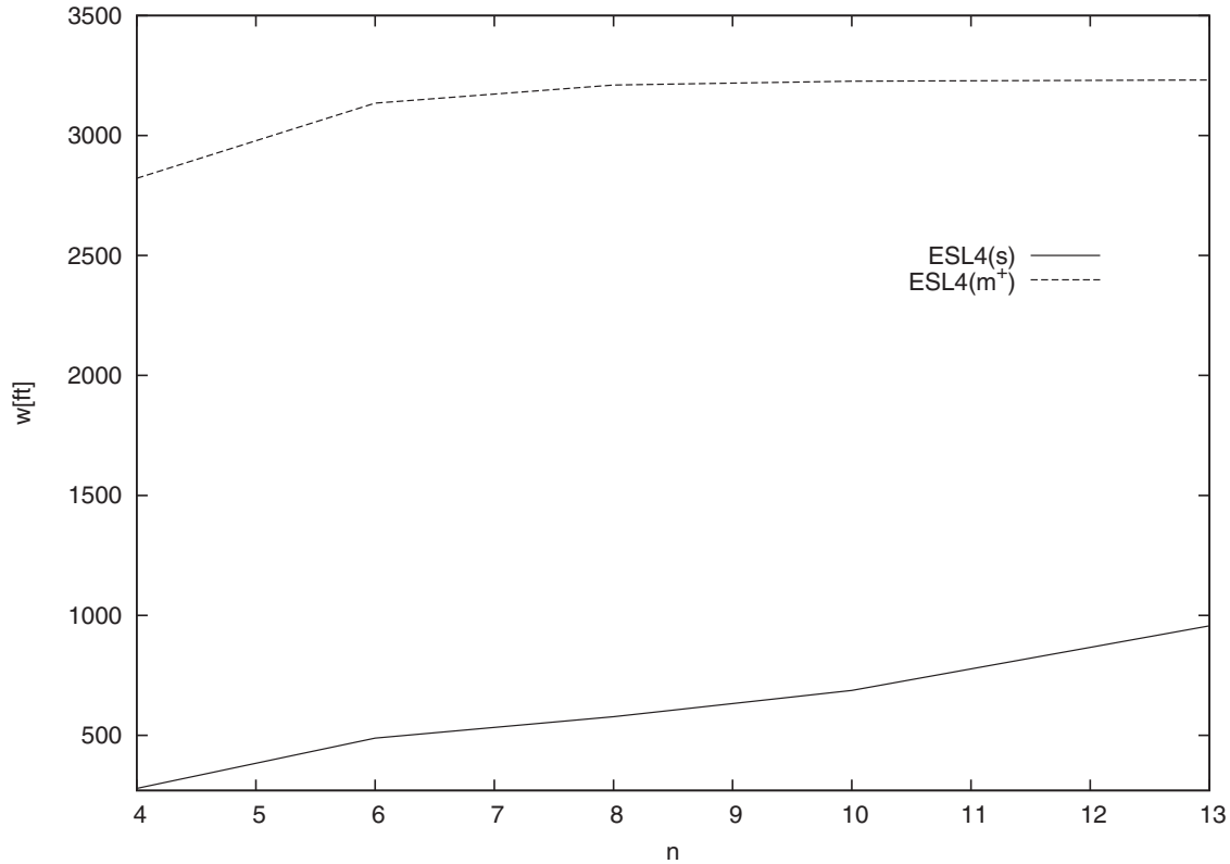
Fig. 8. Scordelis-Lo problem. Thickness ratio t/R = 0.0001 . Transversal displacement w [ft] at the point B of the midsurface S by varying the mesh n \times n .
