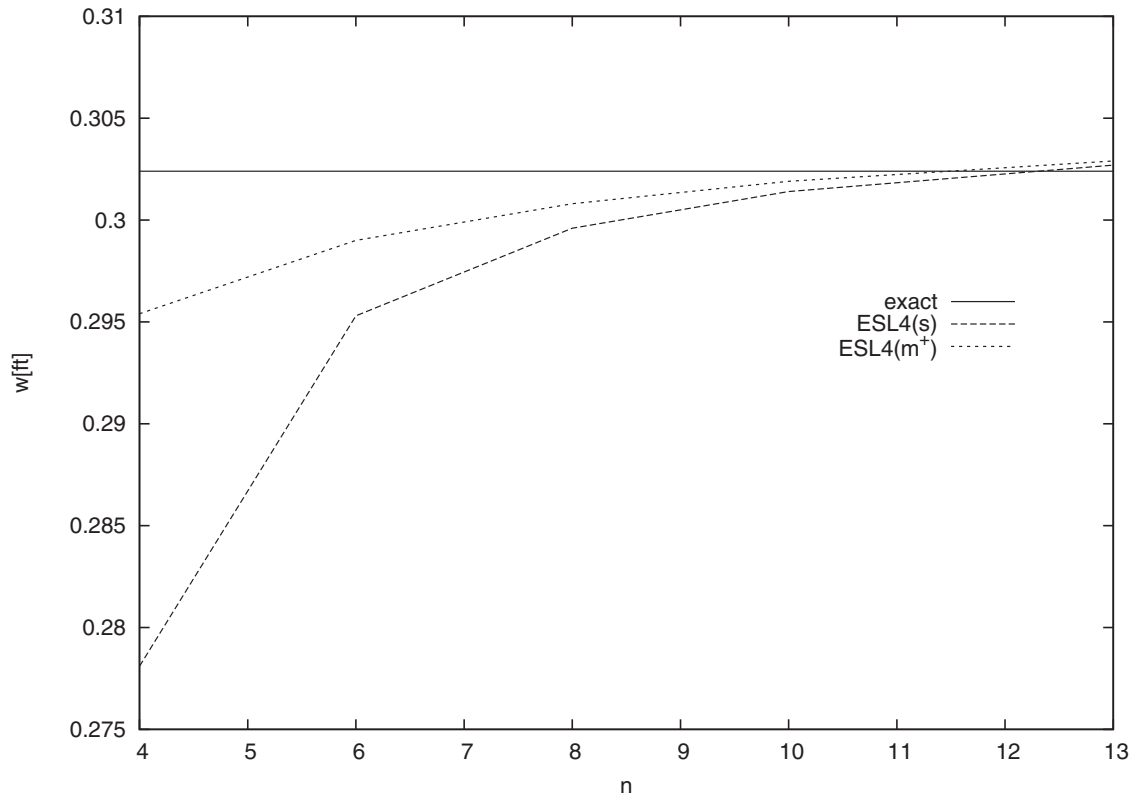
Fig. 6. Scordelis-Lo problem. Thickness ratio t/R = 0.01 . Transversal displacement w [ft] at the point B of the midsurface S by varying the mesh n \times n .
