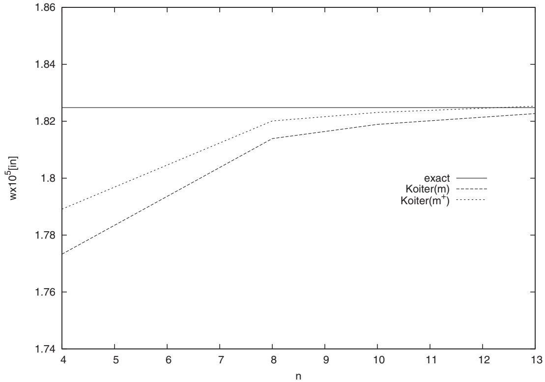
Fig. 4. Pinched shell. Transversal displacement w[\text{in}] \times 10^5 at the loaded point C of the midsurface S by varying the mesh n \times n .
