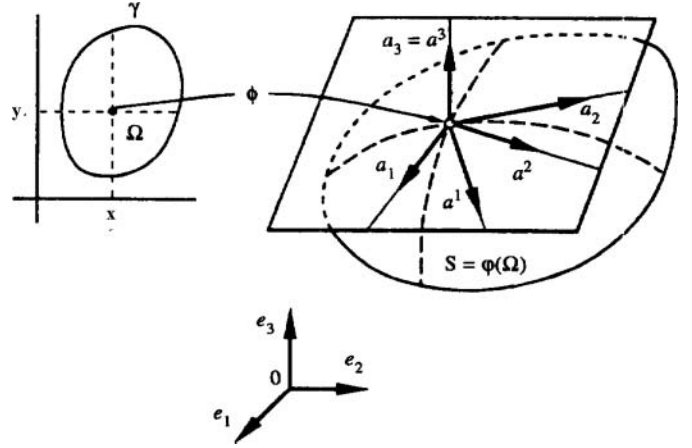
Fig. 1. Definition of the middle surface.
