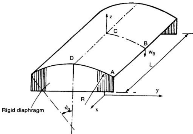
Fig. 5. Scordelis-Lo roof.
