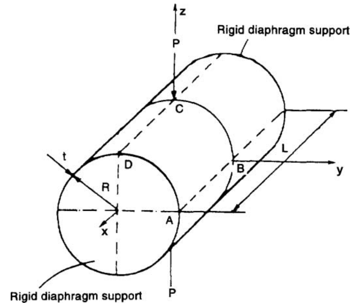
Fig. 3. Pinched shell.
