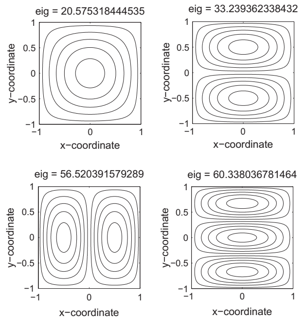
Fig. 4. First four vibrational modes of cross-ply laminated spherical shells, \bar{\omega} = \omega \frac{a^2}{h} \sqrt{\rho/E_2} , laminate ([0°/90°/90°/0°]) grid 13 × 13 points, a/h = 100, R/a = 10.
