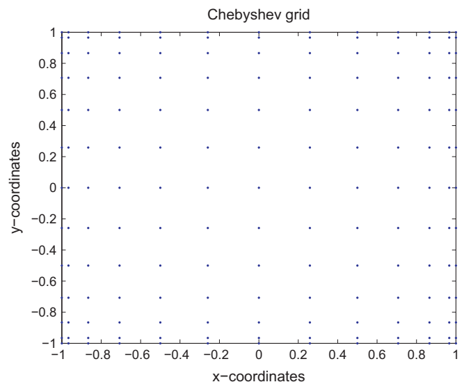
Fig. 3. A sketch of a Chebyshev grid for 13 × 13 points.
